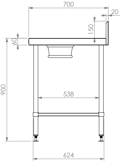
*700mm DEEP MODULE ELEVATION.
