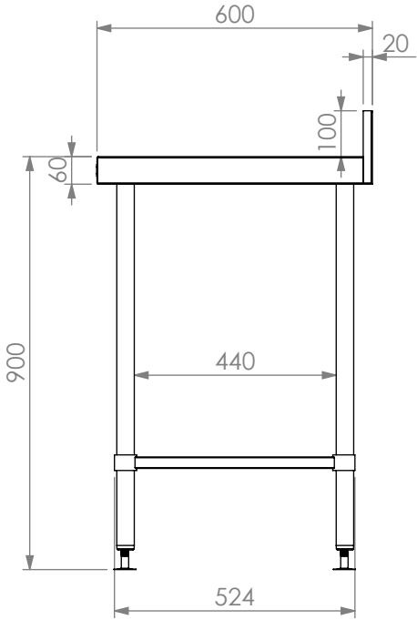
*600mm DEEP MODULE ELEVATION.
